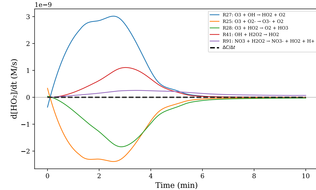
(c) HO 2 [final=13.97 pM]
